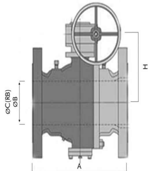
Ball Valve - 2 Pcs. Design (Trunnion Mounted, Gear Operated, Full Bore)
