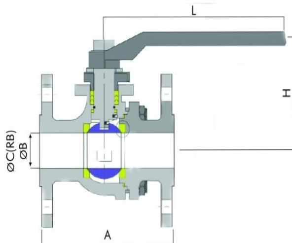
Ball Valve - 2 Pcs. Design (Floating, Lever Operated, Full Bore)
