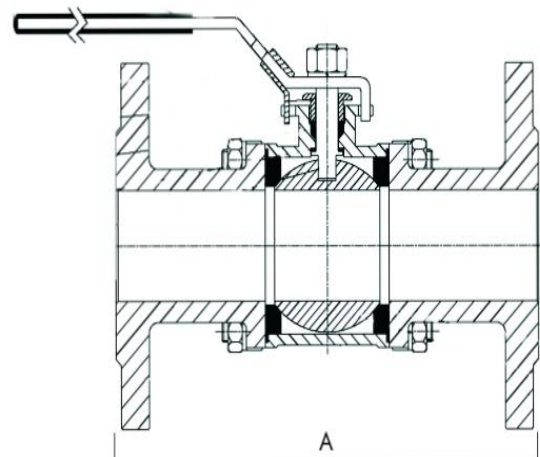
Ball Valve - 3 Pcs. Design (Floating, Lever Operated, Full Bore)
