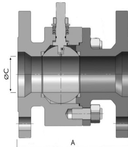
Ball Valve - 2 Pcs. Design (Floating, Lever Operated, Reduce Bore)
